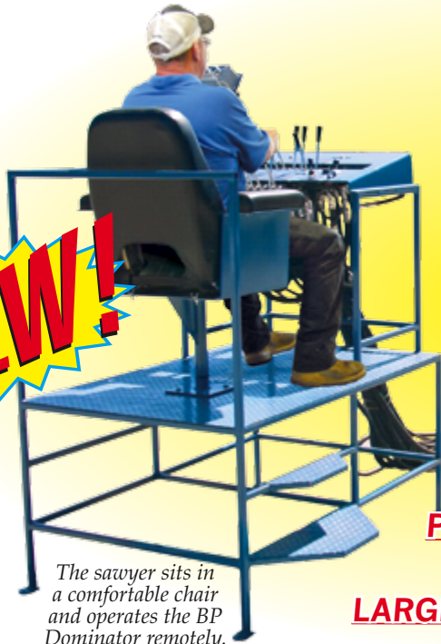
The Model 3650E "BP Dominator" Baker Stationary Band Sawmill
